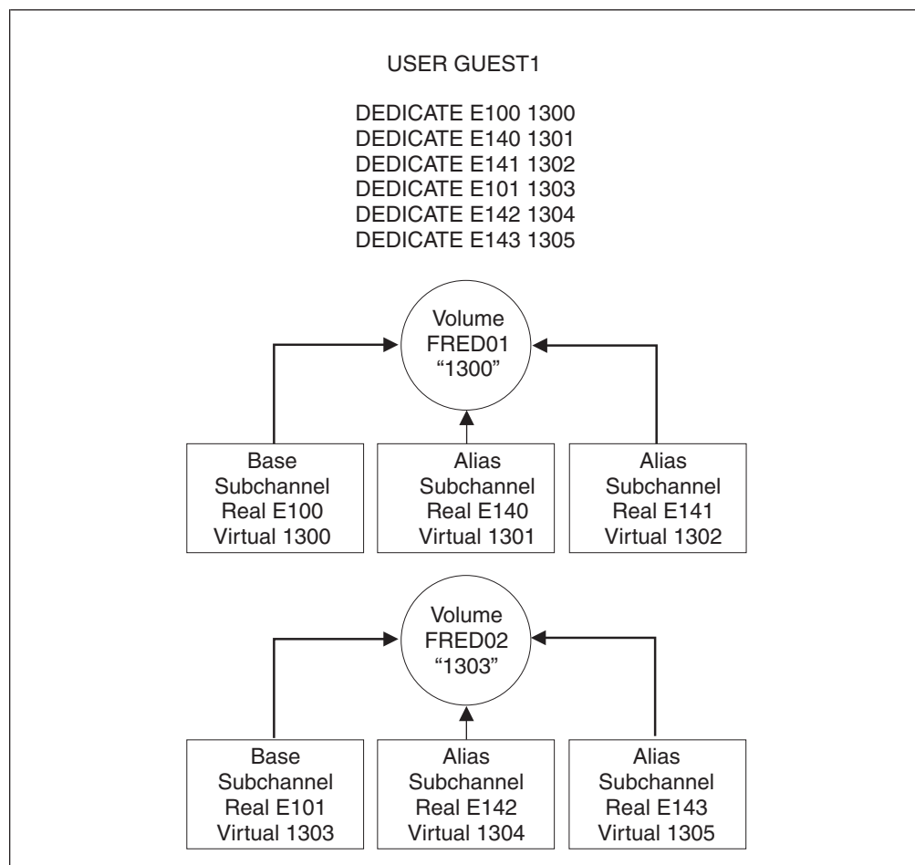
Figure 28. Example: PAV Dedicated Configuration
