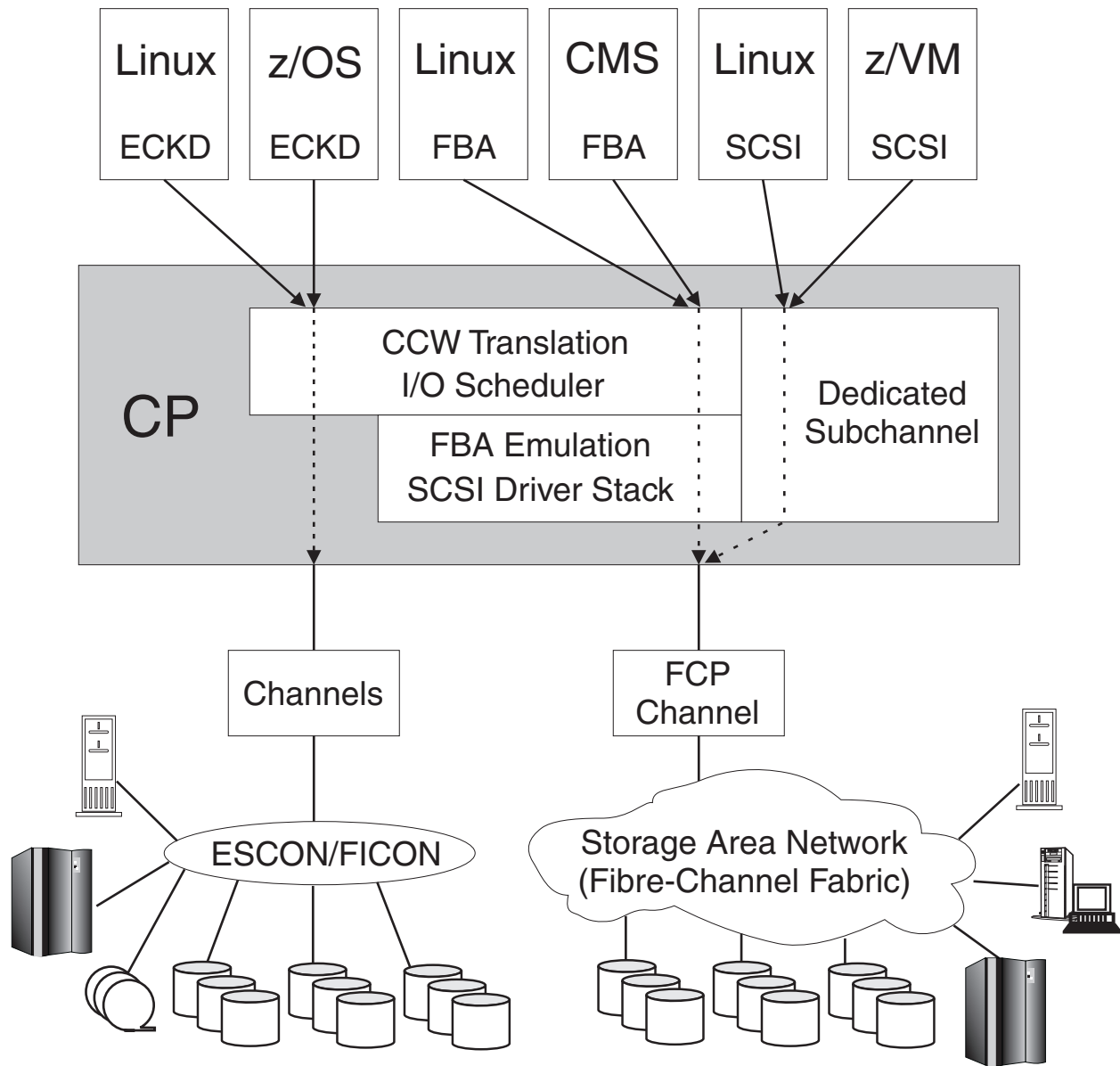
Figure 35. SCSI System Architecture
