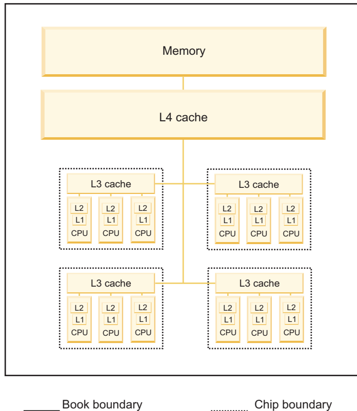
Figure 15. Example of a book with cache structures
