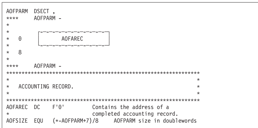
Figure 7. AOFPARM Parameter List for Entry Point HCPACUOF
