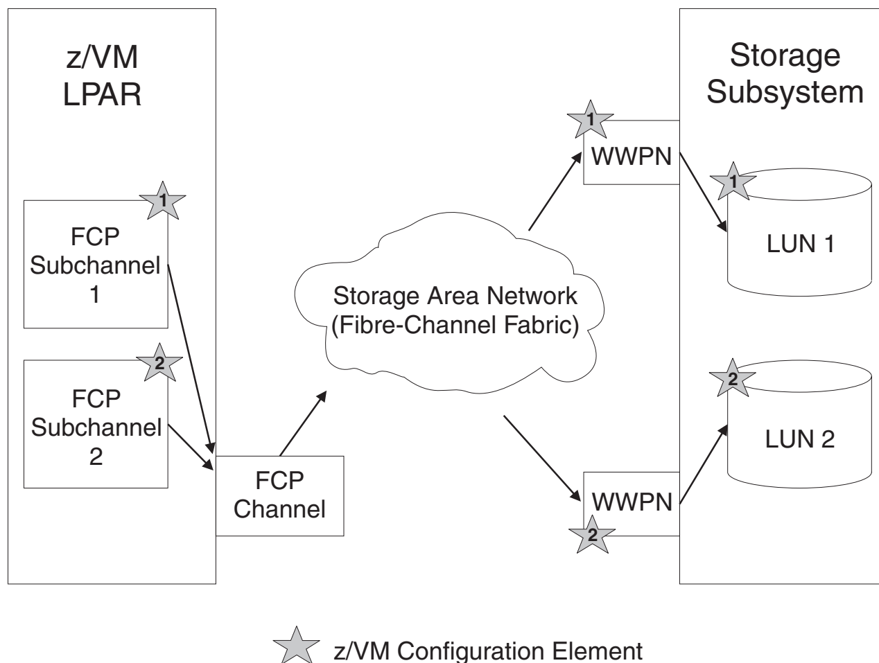
Figure 34. Required Elements for SCSI FCP definition
