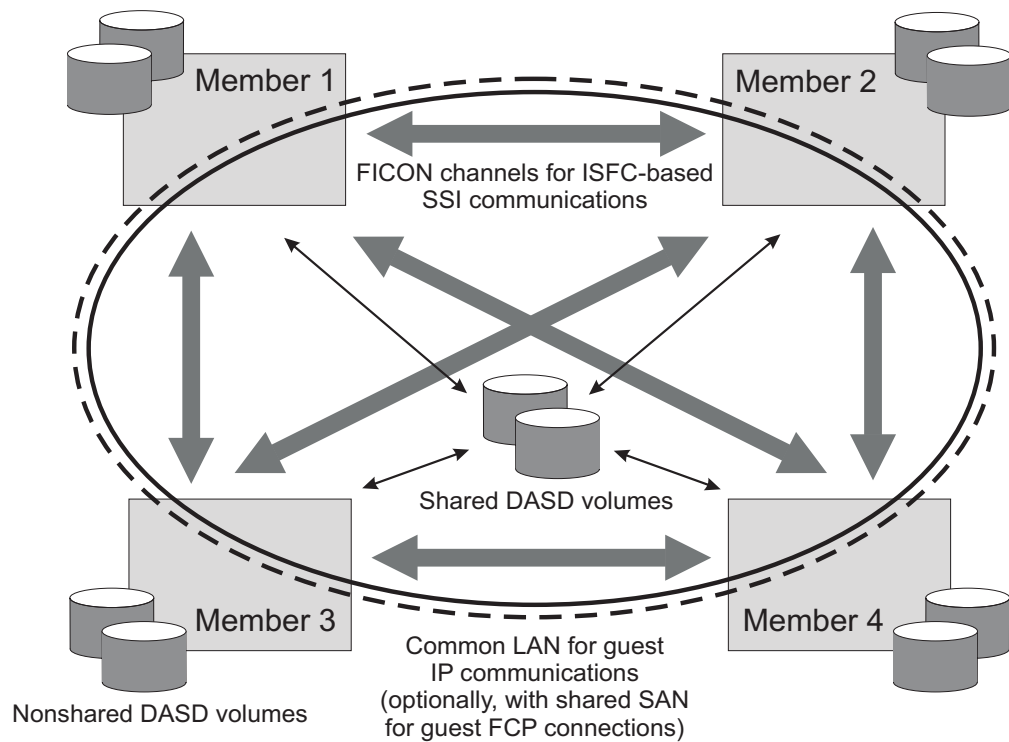
Figure 41. A Four-Member z/VM SSI Cluster
