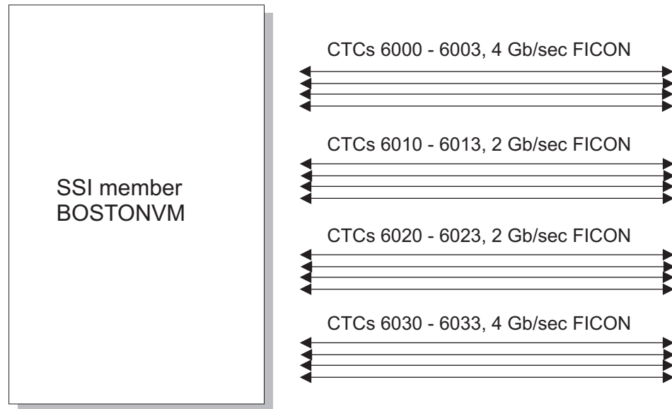
Figure 51. Example of Symmetric Performance with FICON Channel Paths of Differing Speeds
