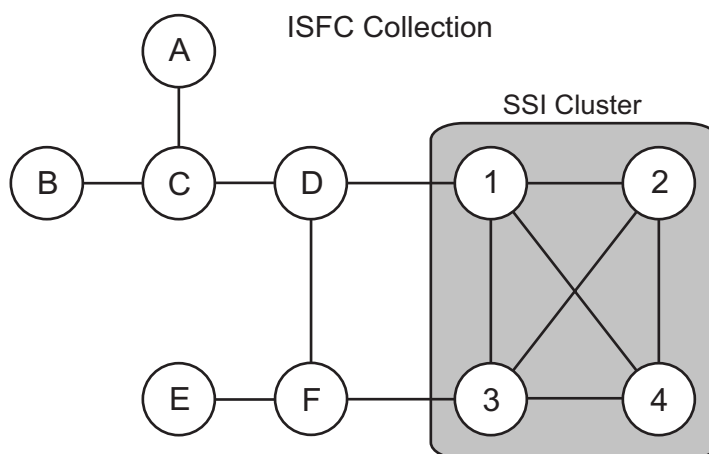
Figure 52. Example of an SSI Cluster within a Larger ISFC Collection
