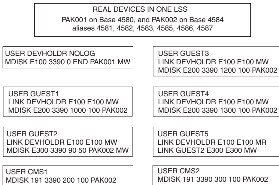
Figure 33. Example: HyperPAV Minidisk Configuration for Non-Exploiting Guests
