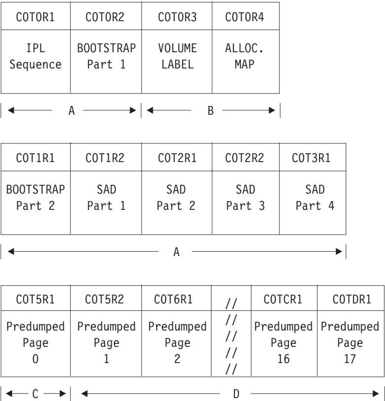
Figure 58. Stand-Alone Dump Facility DASD Format
