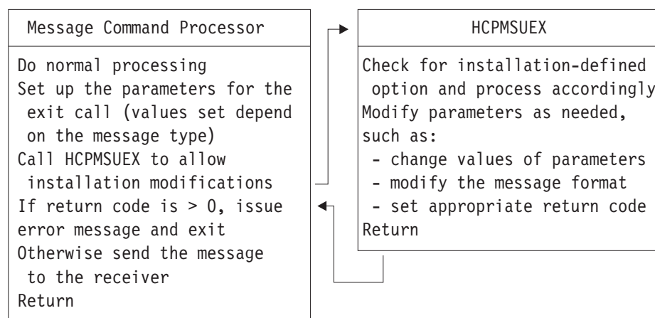
Figure 14. Flow of CP Message Function Customization
